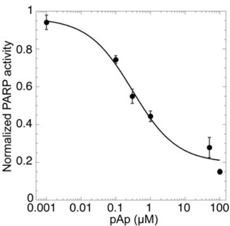
Figure 4 pAp inhibition of histone poly(ADP-ribosyl)ation PARP-1 catalysed poly(ADP-ribosyl)ation of histone H1 was measured as described in the Materials and methods section in the presence of the indicated concentrations of pAp. The PARP-1 activity (arbitrary unit) is expressed as a percentage of the activity in the absence of pAp.
