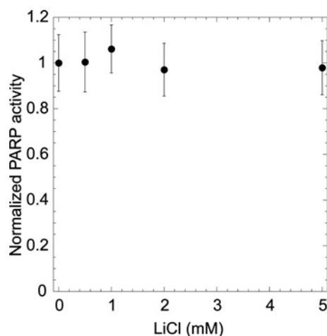
Figure S1 Lithium effect on PARP-1 activity in vitro
