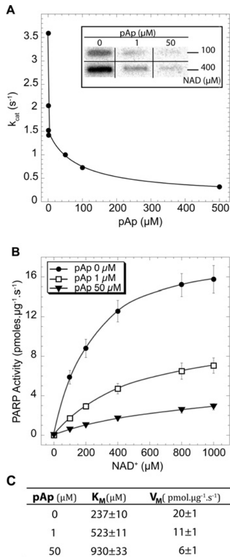
Figure 3 Kinetic parameters of pAp inhibition of PARP-1 activity (A) The k_{cat} , defined as mol of NAD + incorporated/mol of PARP-1 per s, is expressed as a function of the pAp concentration. PARP-1 activity was measured as described in Figure 2. Inset: PhosphorImager autoradiography of poly(ADP-ribosyl)ated PARP-1 blotted on to a nitrocellulose membrane. (B) Activity of PARP-1, expressed as pmol of NAD + incorporated/ \mu g of PARP-1 per s, as a function of the NAD + concentration, and in the presence of the pAp concentrations indicated. For each data point ADP-ribose incorporation was measured at 2, 5, 7 and 10 min. The activity was then determined from the slope of the ADP-ribose incorporated as a function of time. (C) Kinetic parameters of PARP-1 deduced from the results shown in (B).
